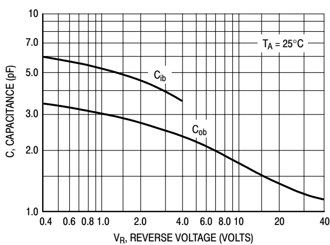
Figure 6. Capacitances
