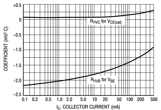
Figure 10. Temperature Coefficients
