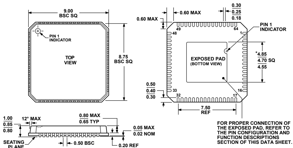
Figure 119. 64-Lead Lead Frame Chip Scale Package [LFCSP_VQ]
