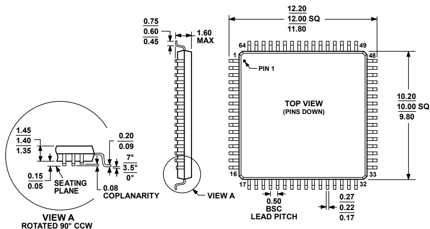
Figure 118. 64-Lead Low Profile Quad Flat Package [LQFP]
