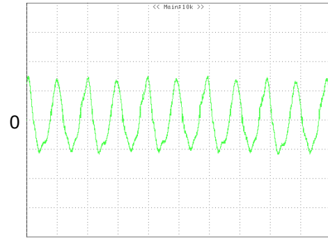
Figure 11: Input Terminal Ripple Current, i_o , at full rated output current and nominal input voltage with 12 \mu H source impedance and 100 \mu F electrolytic capacitor (100 mA/div, 2 \mu s/div)
