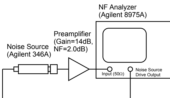
Calibration setup
