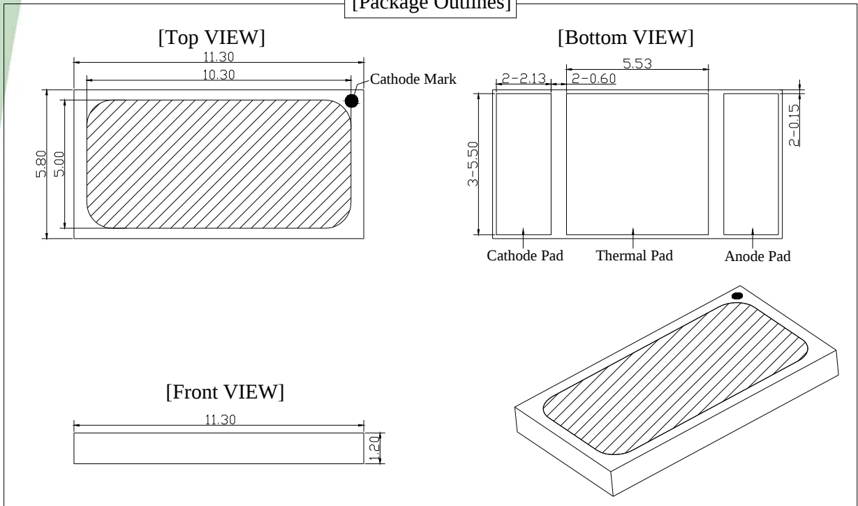
[Package Outlines]
