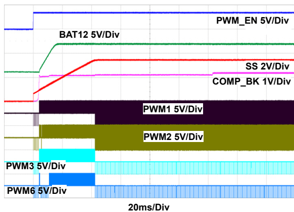
Figure 41. Soft-Start in Buck/FPWM/PD-Enabled, 48V to 12V, 6Ω Load on BAT12
