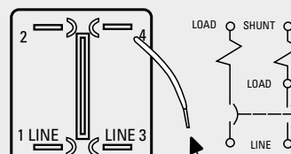
Two Pole ( 1 pole shunt)
