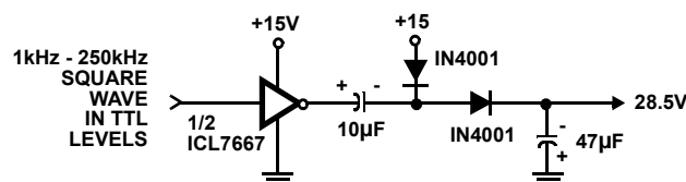
FIGURE 14. VOLTAGE DOUBLER
