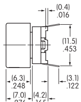
Short Actuator
