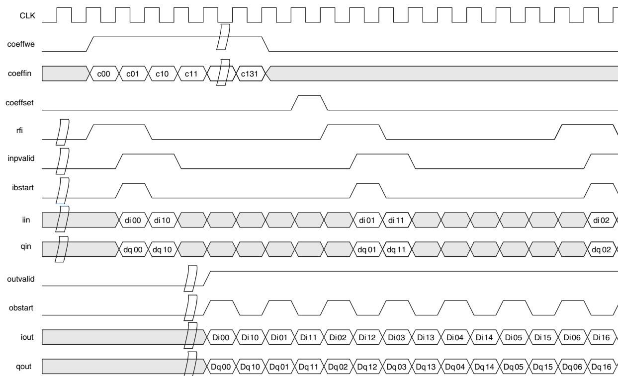
Figure 2-21. Multi-Channel (2 Channels) DHIGHSPEED I&Q Polyphase-Decimator (4:1)
