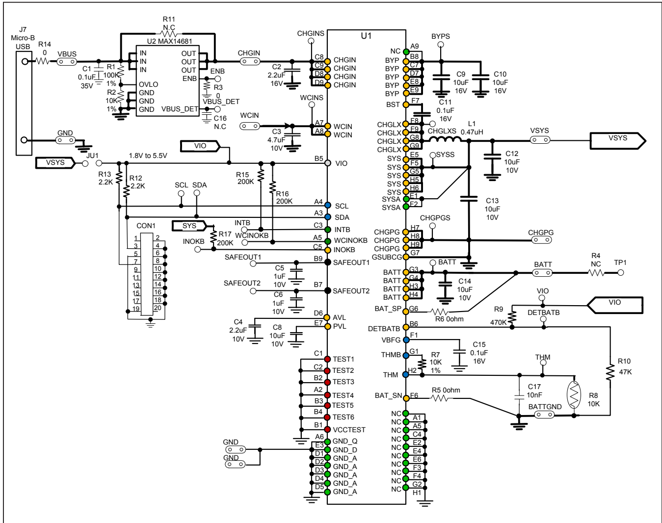
Figure 3. Schematic Diagram
