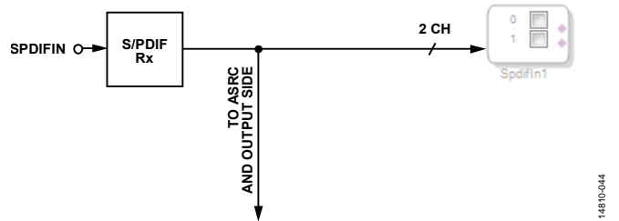
Figure 46. S/PDIF Receiver Direct Input Mapping to DSP in SigmaStudio
