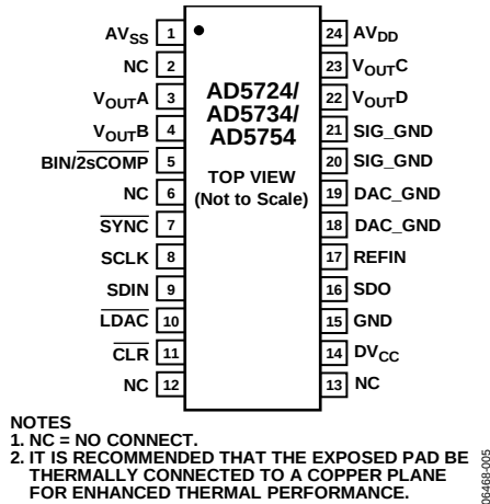
Figure 5. Pin Configuration
