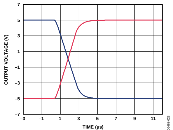
Figure 28. Full-Scale Settling Time, \pm 5\text{V} Range
