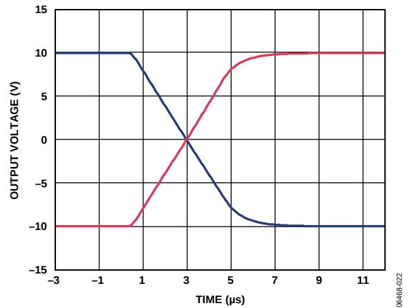
Figure 27. Full-Scale Settling Time, \pm 10\text{V} Range
