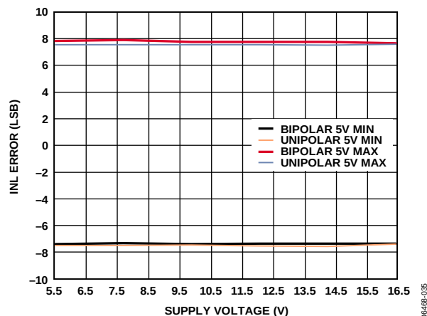
Figure 15. AD5754 INL Error vs. Supply Voltage
