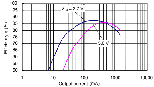
(4) S-8533A33AFT (Si3441DV/Si3442DV)
