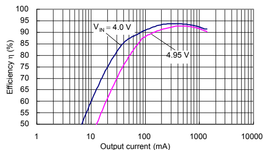
(22) S-8533A33AFT (Si3454DV/Si3455DV)
