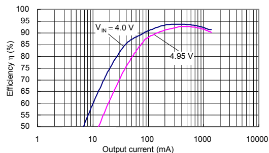
(22) S-8533A33AFT (Si3454DV/Si3455DV)
