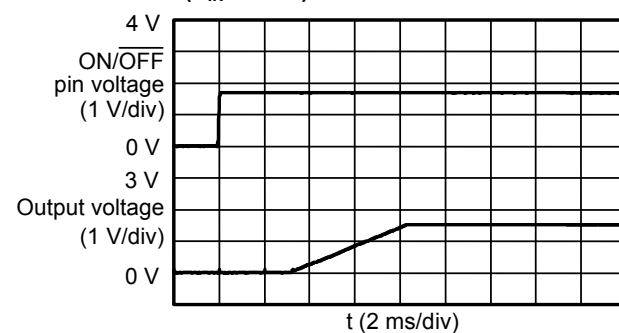
S-8533A33AFT ( V_{IN} : 9.0\text{ V} )
