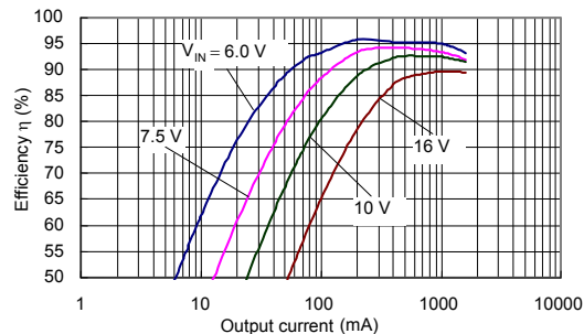
(24) S-8533A50AFT (Si3454DV/Si3455DV)
