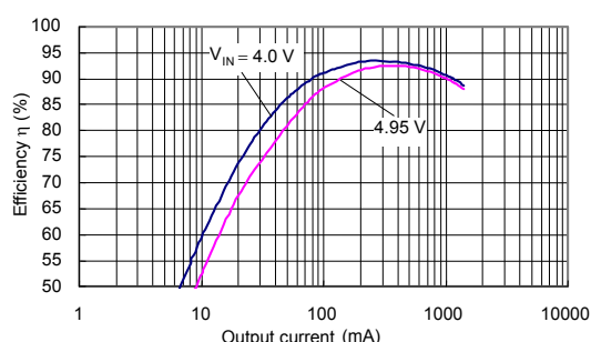
(14) S-8533A33AFT (Si3454DV/Si3455DV)
