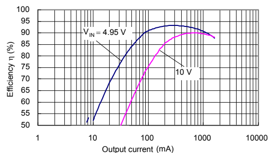
(24) S-8533A50AFT (Si3454DV/Si3455DV)
