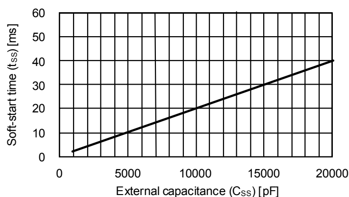
Figure 7 Soft-Start Time
