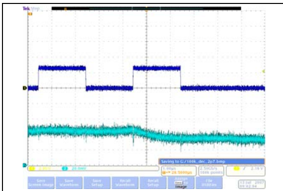
FIGURE 2-51: 100\text{ k}\Omega – Low-Voltage Decrement Wiper Settling Time ( V_{DD} = 2.7\text{V} ) ( 1\text{ }\mu\text{s}/\text{Div} ).
