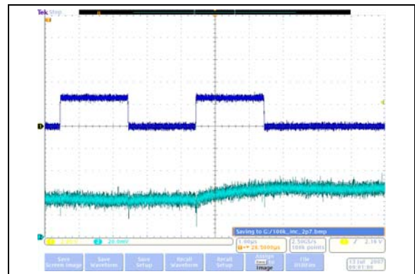
FIGURE 2-53: 100\text{ k}\Omega – Power-Up Wiper Response Time ( 1\text{ }\mu\text{s}/\text{Div} ).
