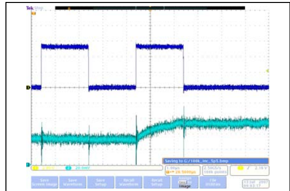
FIGURE 2-52: 100\text{ k}\Omega – Low-Voltage Increment Wiper Settling Time ( V_{DD} = 2.7\text{V} ) ( 1\text{ }\mu\text{s}/\text{Div} ).
