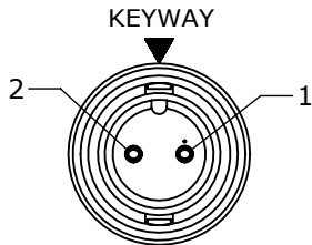
FACE VIEW P/N: CA62802SXXX90
