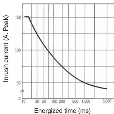
G3NE-210T(L)(-2)-US
