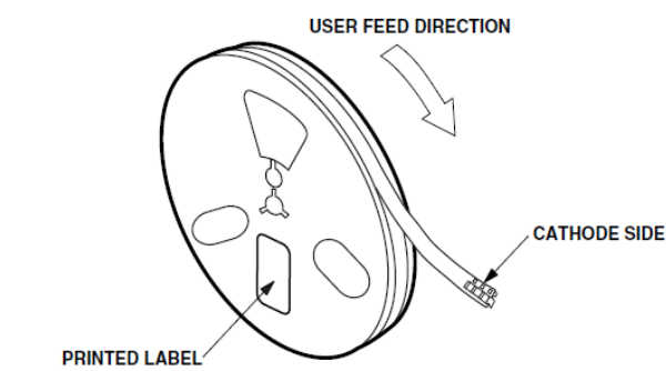
Figure 12: Reel Orientation
