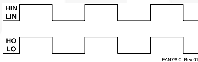
Figure 27. Input/Output Timing Diagram
