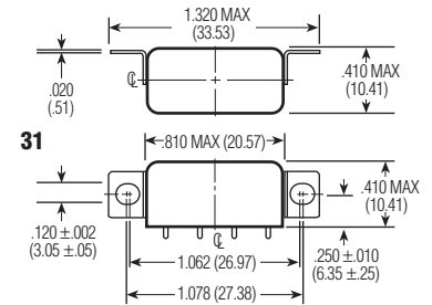
Mounting Styles
