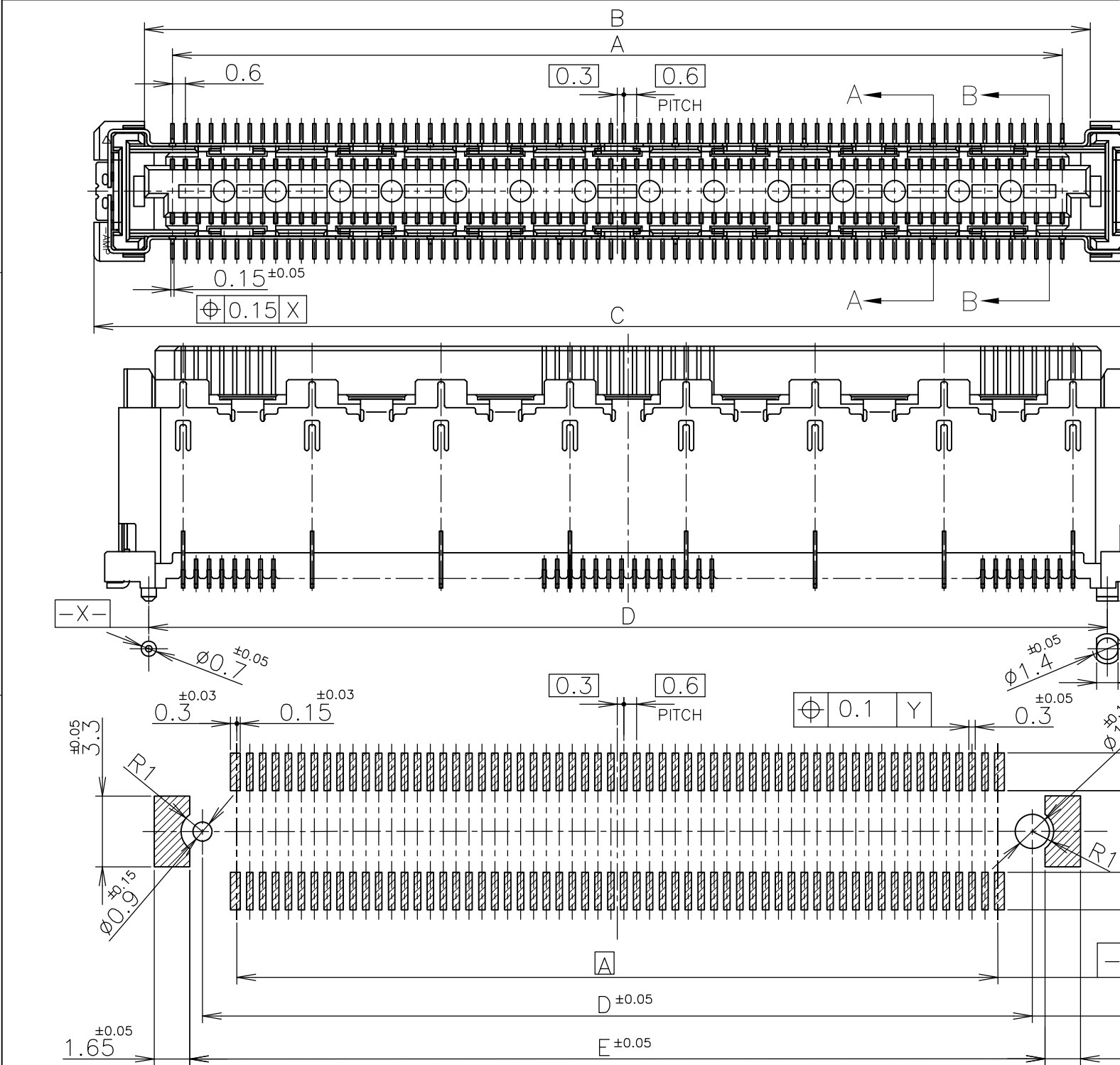
REFERENCE P.C. BOARD LAYOUT
