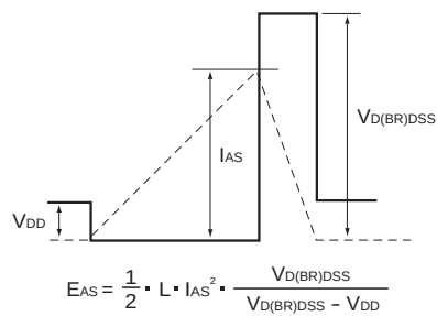
Fig.3-2 Avalanche waveform
