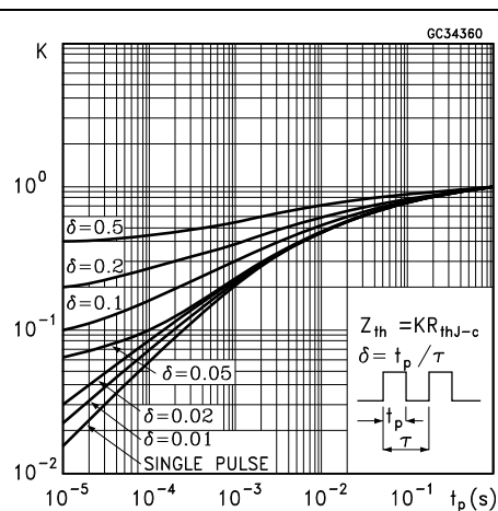
Figure 3. Thermal impedance for DPAK and IPAK
