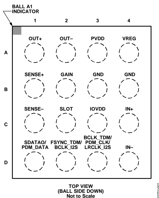
Figure 2. Pin Configuration
