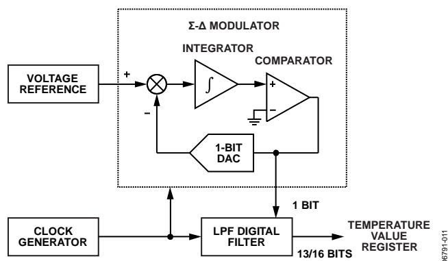
Figure 10. \Sigma - \Delta Modulator
