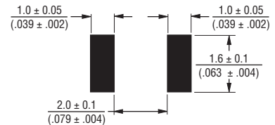
Recommended Pad Layout
