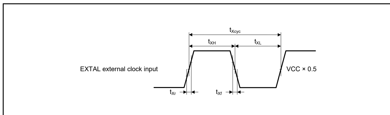
Figure 5.20 EXTAL External Clock Input Timing
