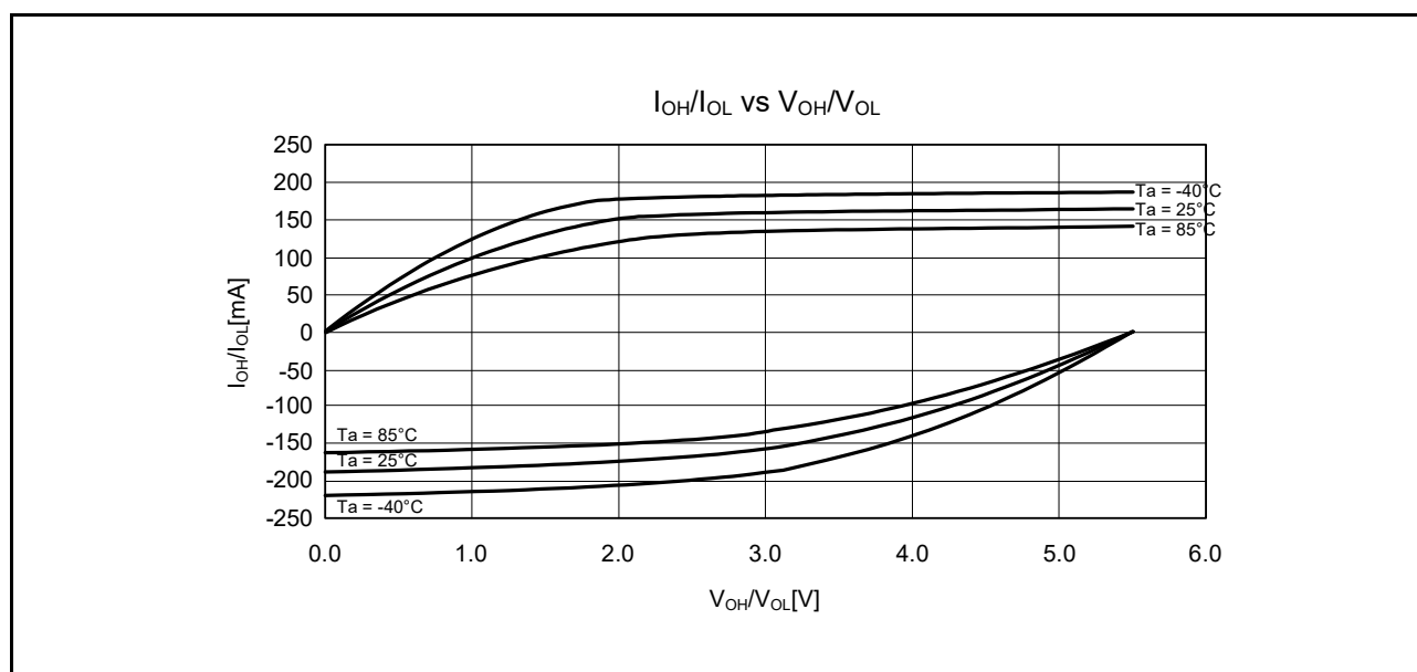
Figure 5.15 V_{OH}/V_{OL} and I_{OH}/I_{OL} Temperature Characteristics of Large Current Ports at V_{CC} = 5.5\text{ V} (Reference Data)
