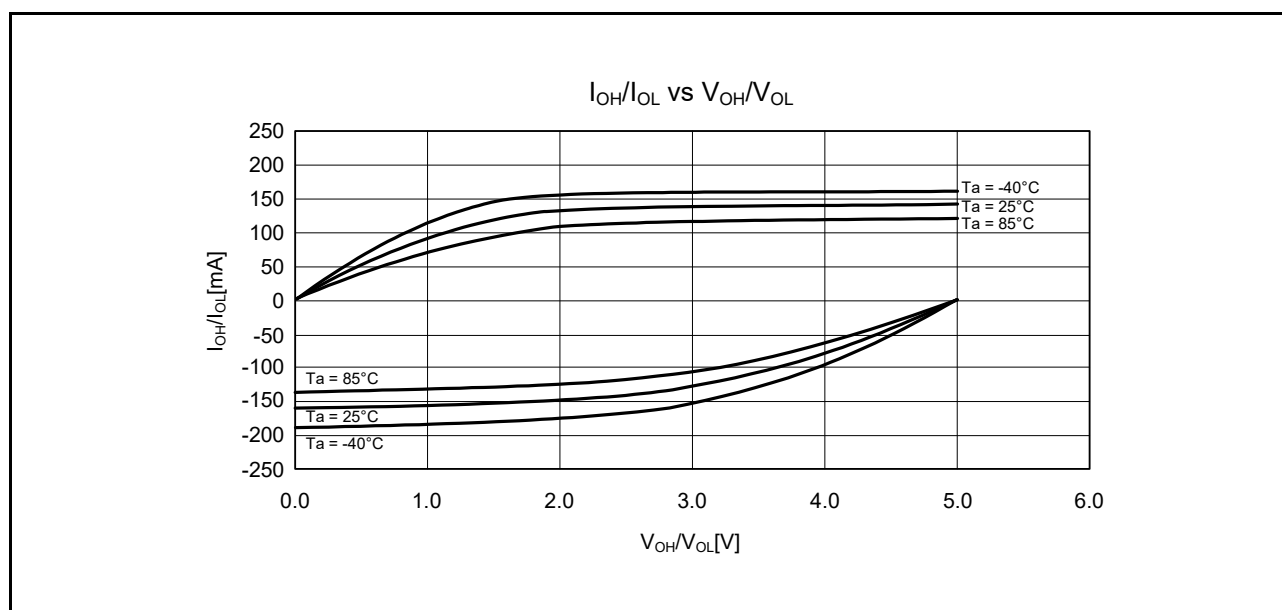
Figure 5.14 V_{OH}/V_{OL} and I_{OH}/I_{OL} Temperature Characteristics of Large Current Ports at V_{CC} = 5.0\text{ V} (Reference Data)
