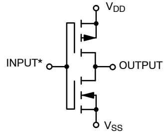
Figure 2. Circuit Schematic
