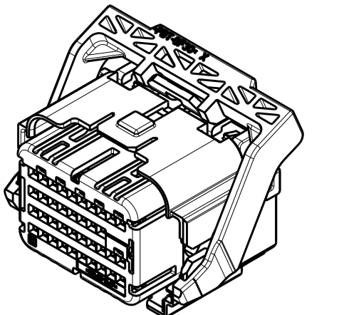
KEYING OPTION "G" SHOWN SEE SHEET 2 FOR BILL OF MATERIALS AND SHEET 3 FOR PIN-OUT CHARTS
