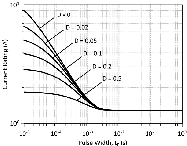
Figure 5: Current vs Pulse Duration Curves at T_C = 225 \text{ °C}
