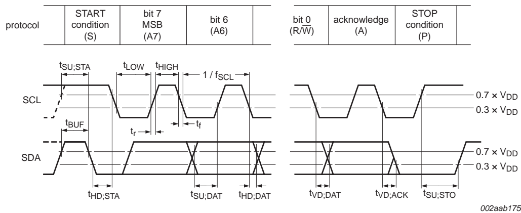
Fig 16. I 2 C-bus timing diagram
