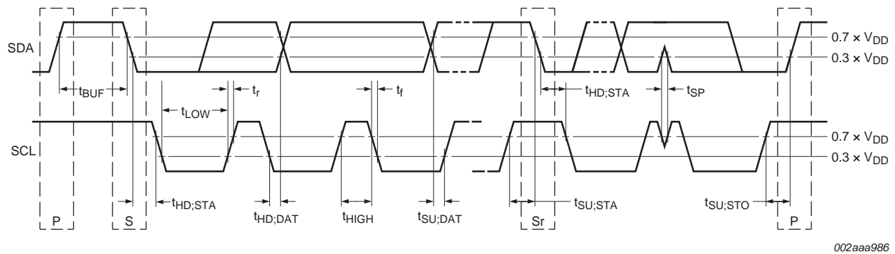
Fig 15. Definition of timing
