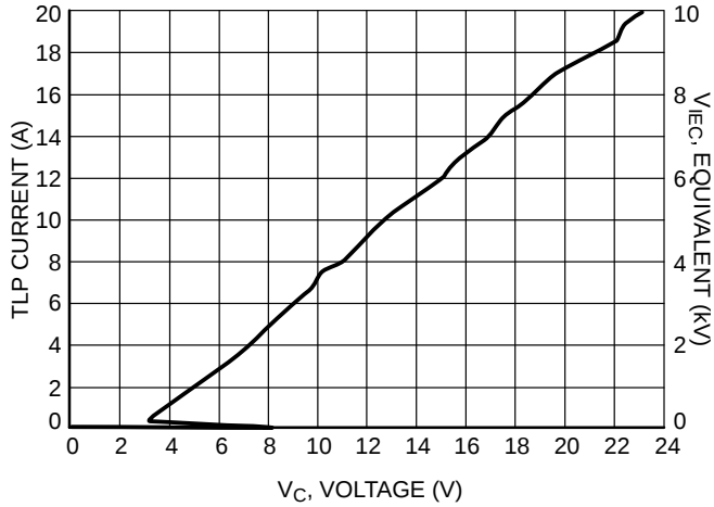
Figure 7. ESD8451MUT5G Positive TLP I-V Curve
