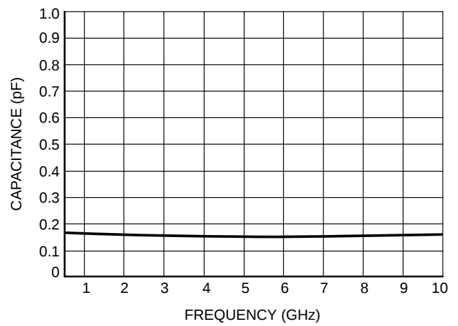
Figure 6. ESD8451N2T5G Capacitance over Frequency
