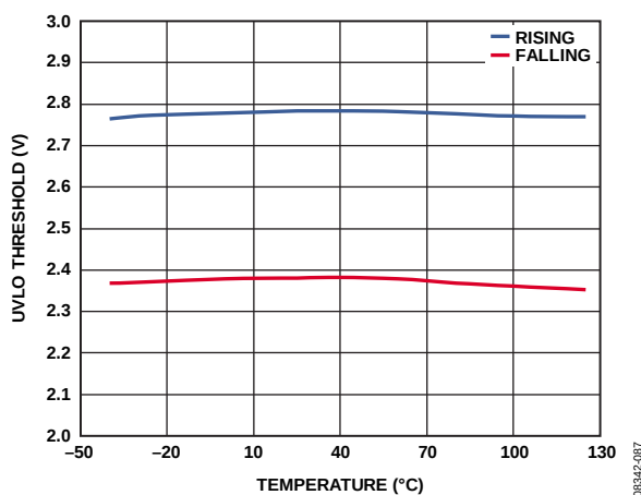
Figure 25. UVLO Threshold vs. Temperature
