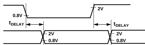
Figure 3. Voltage Reference Levels for Timing
