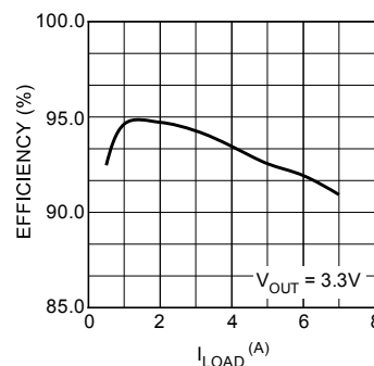
Efficiency for V IN = 5V and V OUT = 3.3V
