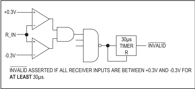
Figure 3a. INVALID Functional Diagram, INVALID Low
