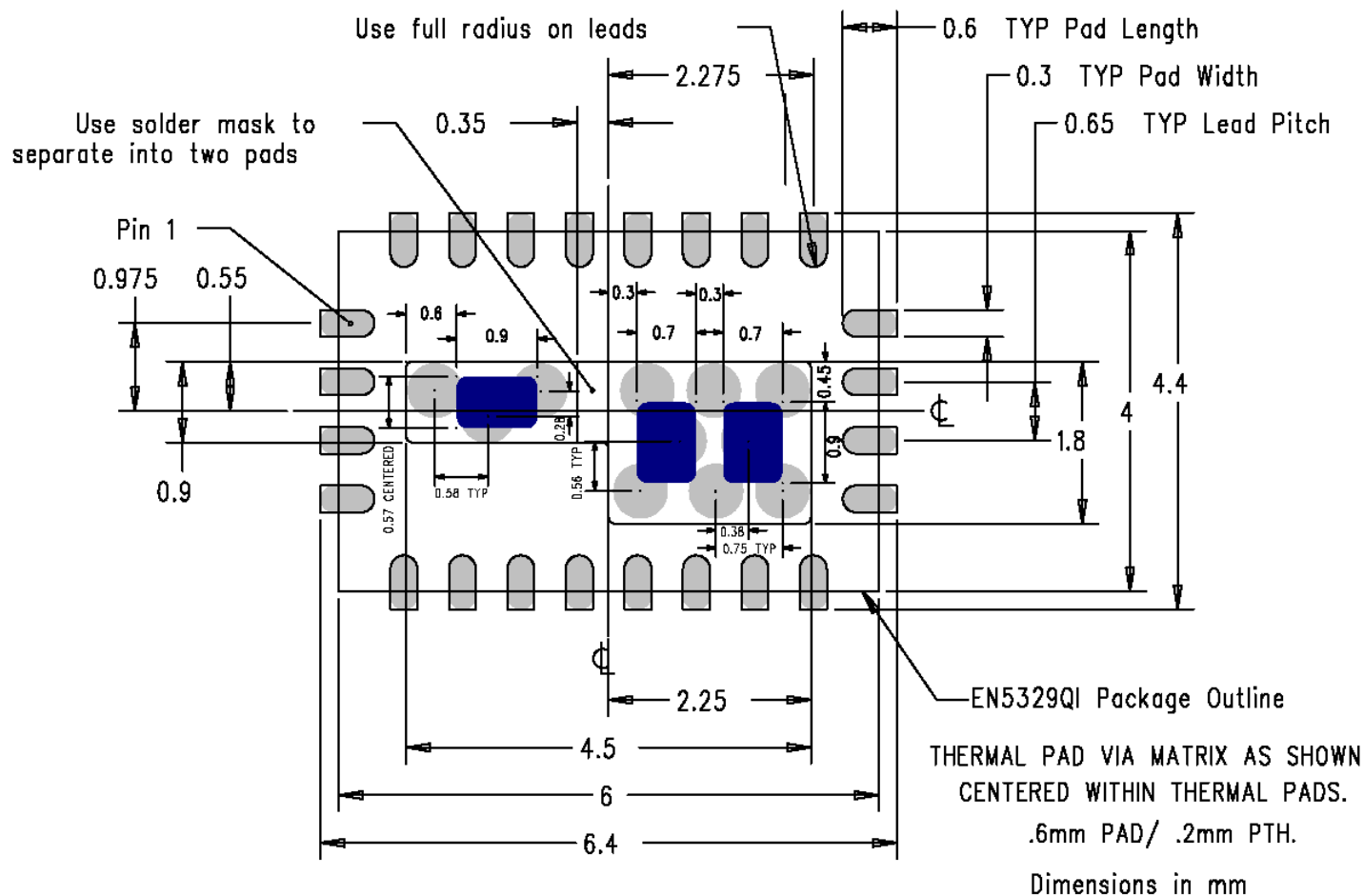
Figure 11: Landing Pattern with Solder Stencil (Top View)
