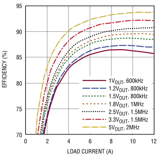
c) 12V IN CCM Efficiency vs Load Current
