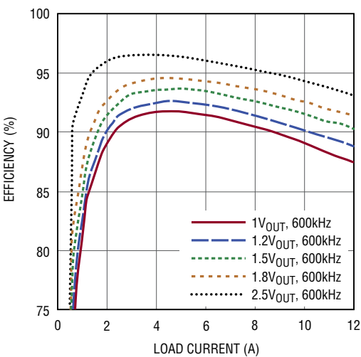
a) 3.3V IN CCM Efficiency vs Load Current
