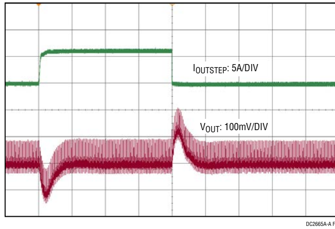
Figure 3. Load Transient (6A to 12A) Response Waveform at 12V IN and 1.5V OUT , 50 \mu s/DIV
