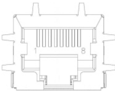
Figure 8. RJ-45 Connector
