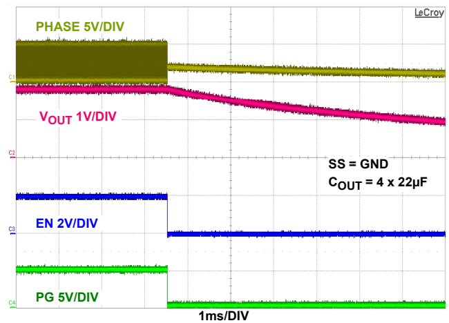
FIGURE 20. \text{EN} SHUTDOWN AT NO LOAD ( \text{SYNC} = V_{DD} )
