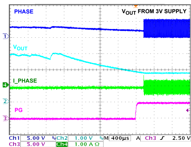
FIGURE 41. OVERVOLTAGE RECOVERY
