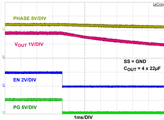
FIGURE 19. \text{EN} SHUTDOWN AT NO LOAD ( \text{SYNC} = \text{GND} )
