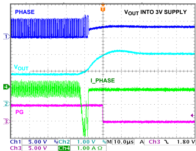
FIGURE 40. OVERVOLTAGE PROTECTION
