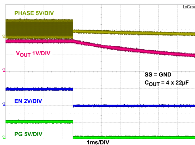
FIGURE 20. \text{EN} SHUTDOWN AT NO LOAD ( \text{SYNC} = V_{DD} )
