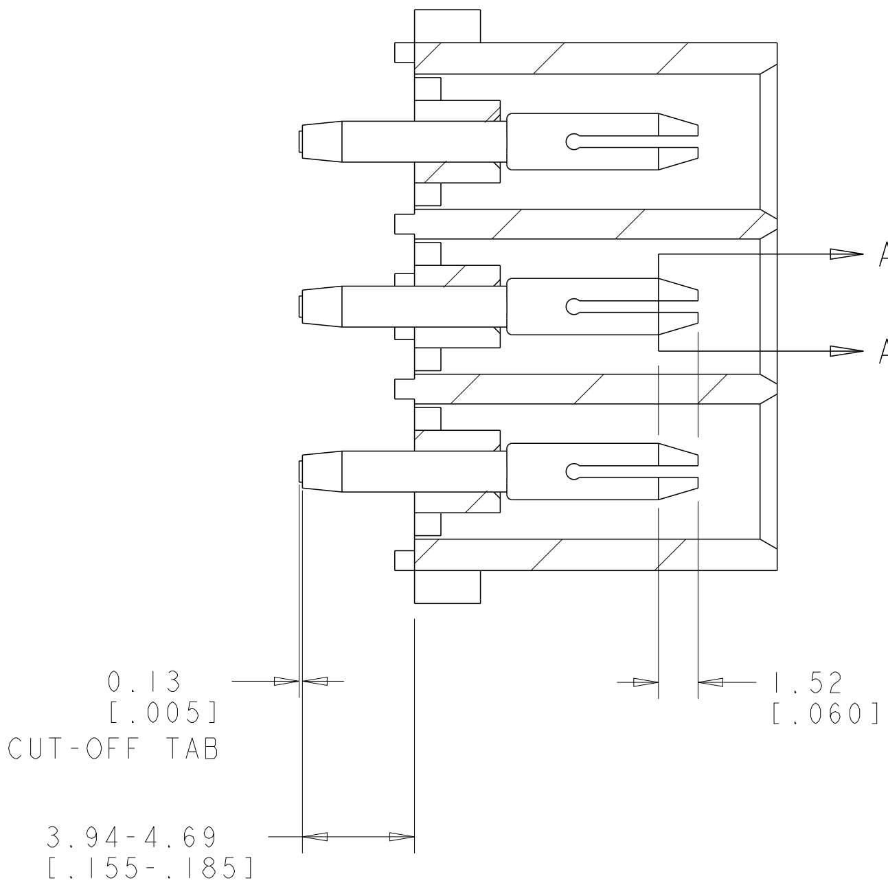
SECTION B-B
