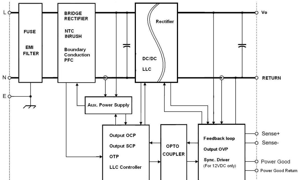
Figure 1. ABC200-10XXG block diagram
